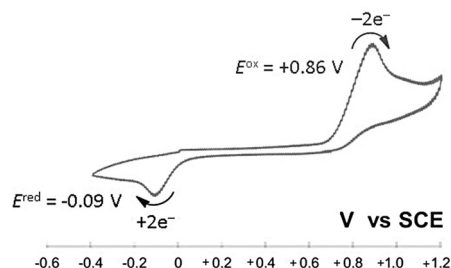
Figure 1. Cyclic voltammogram of 1 measured in \text{CH}_2\text{Cl}_2 (E/V vs. SCE, Pt electrode, scan rate 500 mV s -1 ).
